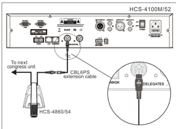
Figure 3.8.2 HCS-4860/54 series congress unit connected to the CMU/EMU
