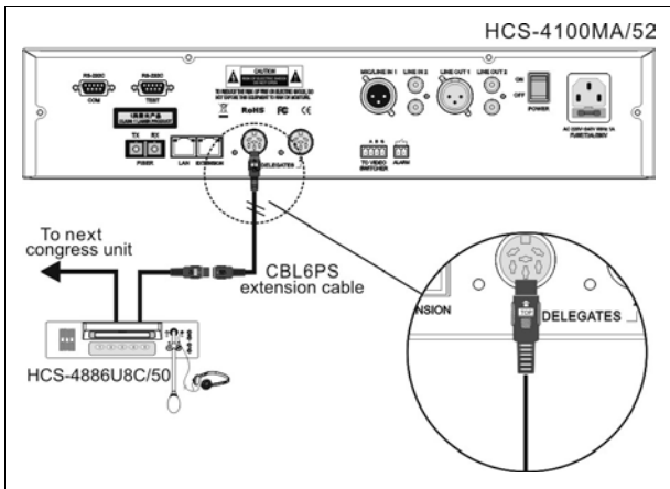
Figure 3.3.12 HCS-48U7/U8/U9 series congress unit connected to the CMU/EMU
