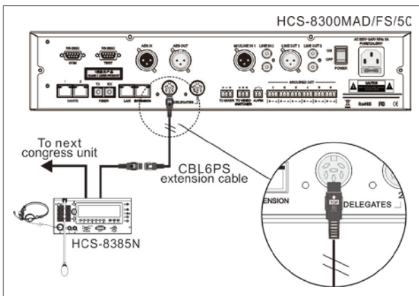
Figure 4.2.1 HCS-8385N Interpreter unit connected to the CMU or the EMU
