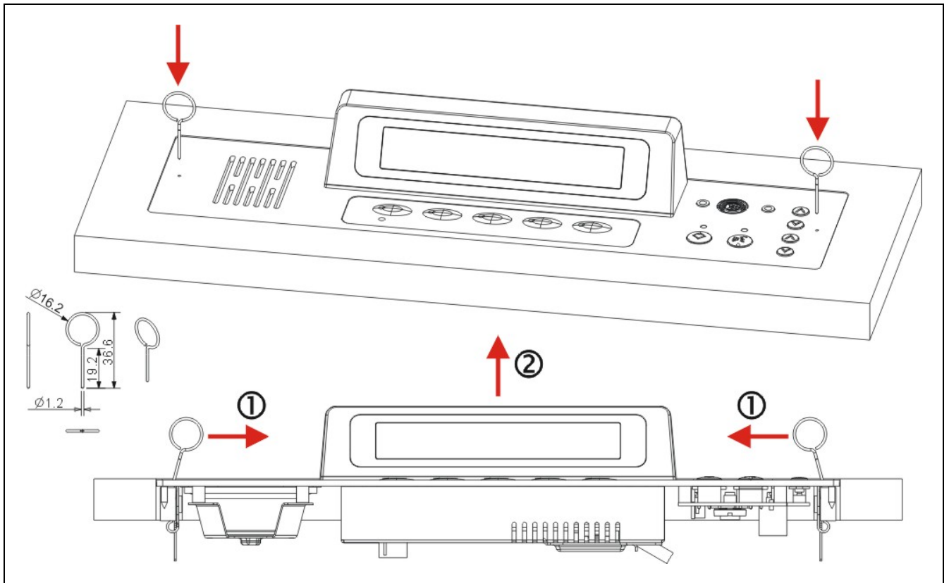
Figure 3.3.7 Disassembly of HCS-48U8 and HCS-48U9 series flush-mounted congress unit (method a)
