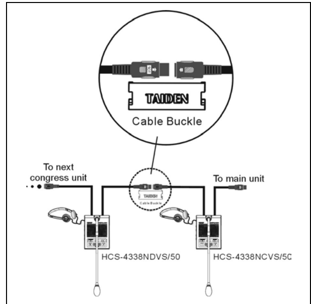
Figure 3.7.3 “Daisy-chain” connection between HCS-4338N/50 series congress units
