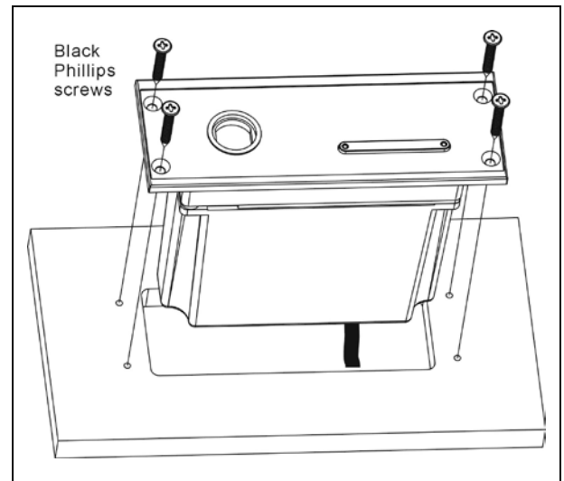
Figure 3.10.4 Installation diagram of HCS-4841N series congress unit (unit: mm)
