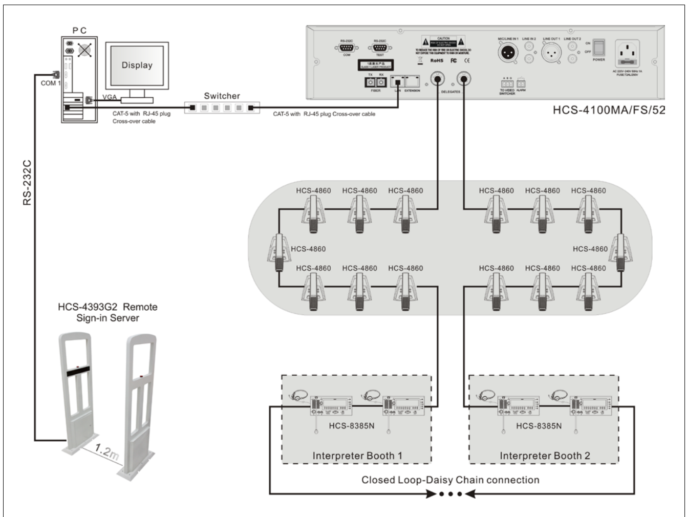
Figure 5.1.6 Connection between Conference Sign-in System and HCS-4100/50 system
