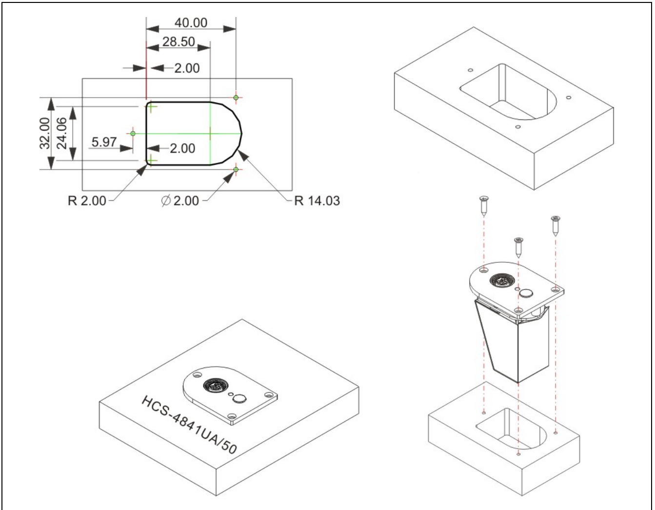
Figure 3.10.6 Installation of the HCS-4841UA/50 flush-mounted channel selector
