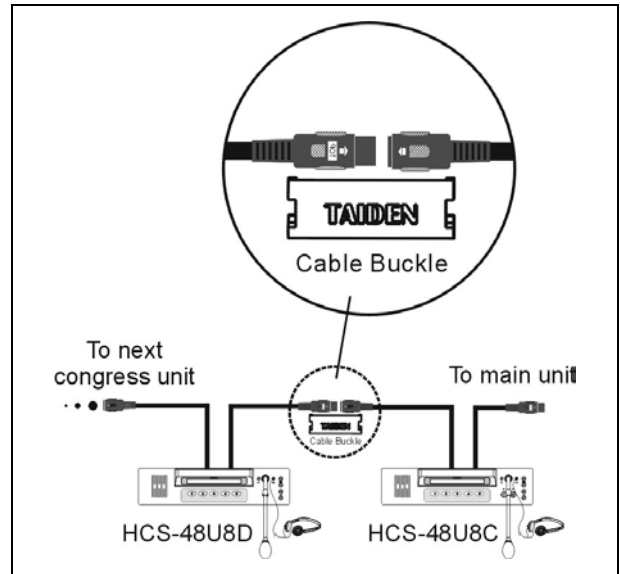
Figure 3.3.13 “Daisy-chain” connection between HCS-48U7/U8/U9 series congress units
