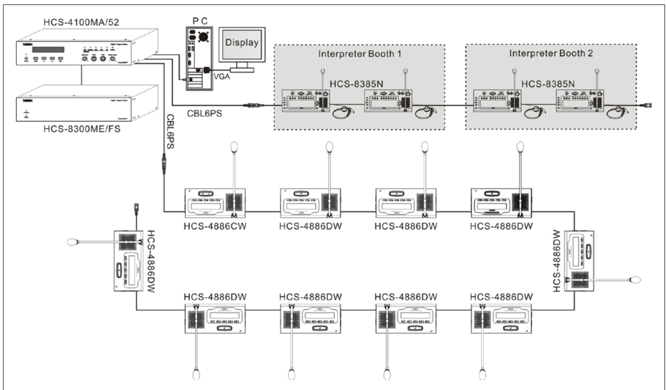
Figure 1.1.1 System overview
