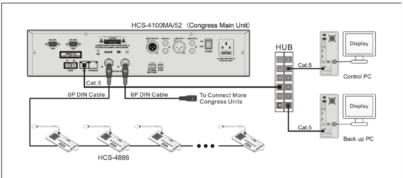
Figure 5.1.9 Dual PC server hot spare
