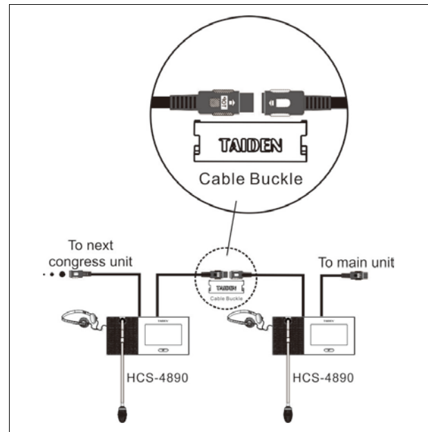
Figure 3.6.3 “Daisy-chain” connection between HCS-4890/52 series congress units
