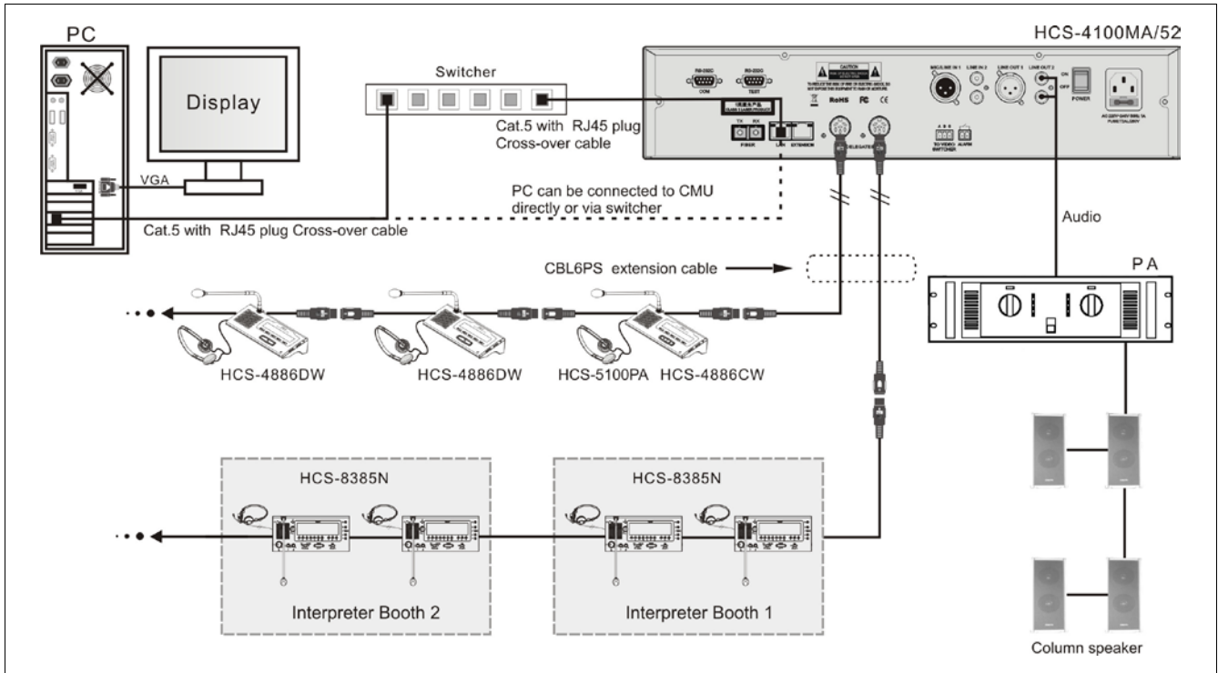
Figure 5.1.1 Congress main unit connecting to HCS-4886 series contribution units and HCS-8385N interpreter units
