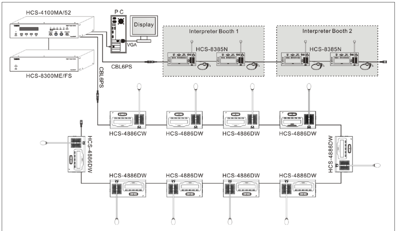
Figure 5.2.1 Connection example of HCS-4100/50 system
