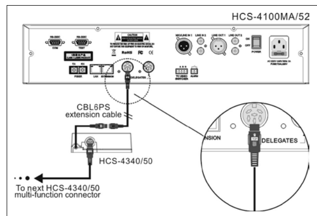
Figure 3.9.3 HCS-4340/50 series multi-function connector connected to the CMU/EMU
