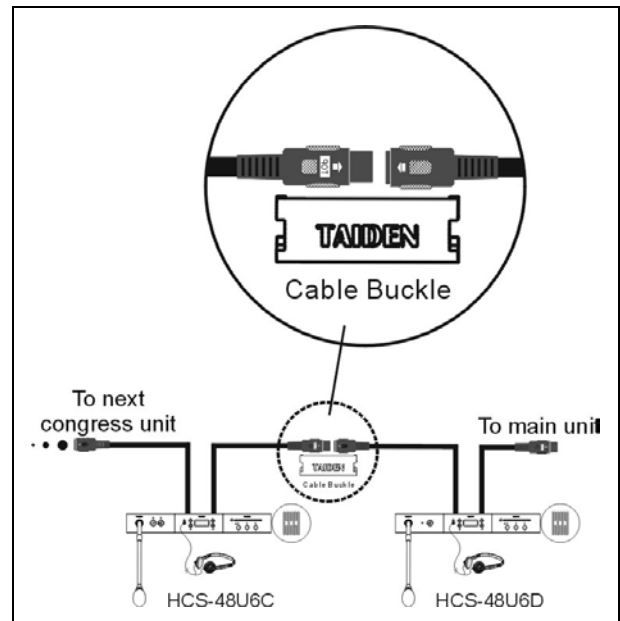
Figure 3.2.9 “Daisy-chain” connection between HCS-48U6 series congress unit
