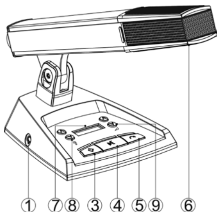
HCS-4860CS/54 chairman unit HCS-4860CS/54/2M chairman unit
