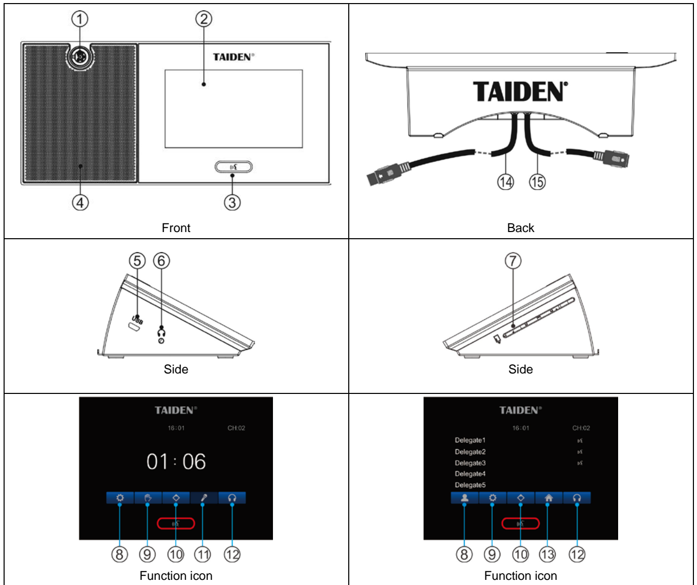
Figure 3.6.1a HCS-4890/52 series congress units
