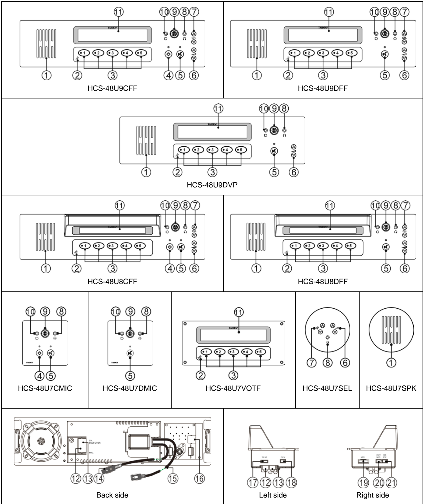
Figure 3.3.1 HCS-48U7/U8/U9 series congress units
