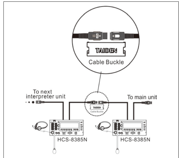
Figure 4.2.2 “Daisy-chain” connection between HCS-8385N Interpreter units
