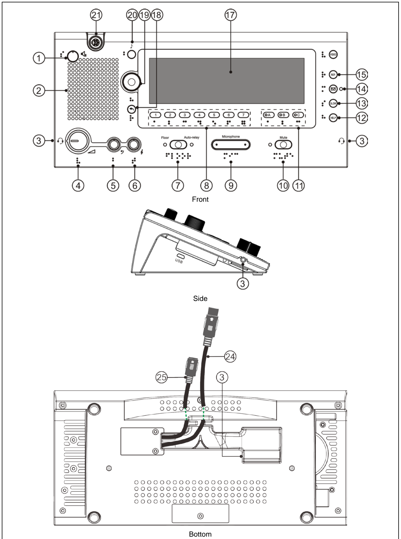
Figure 4.1.1 HCS-8385N Interpreter unit
