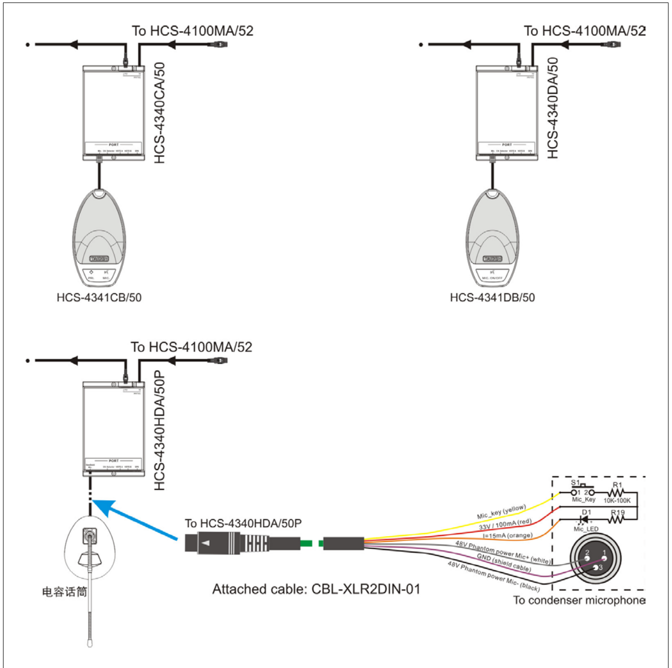
Figure 3.9.5 Multi-function connector connected to the HCS-4341/50 series congress unit
