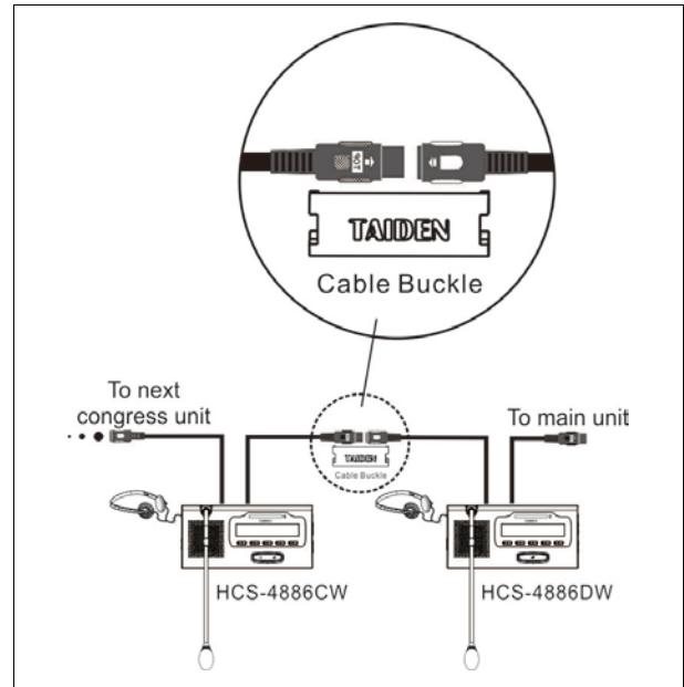
Figure 3.5.4 “Daisy-chain” connection between HCS-4886 series congress units
