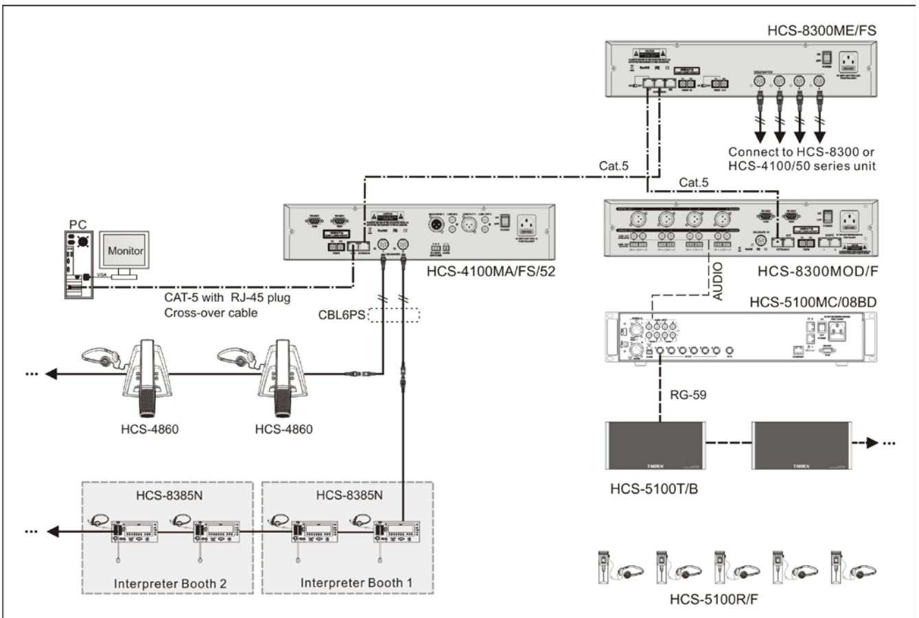
Figure 5.1.4 Congress main unit connecting to digital infrared language distribution system via HCS-5100MC/B
