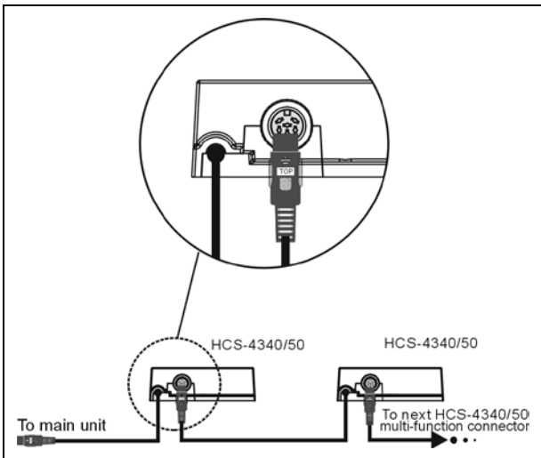
Figure 3.10.8 “Daisy-chain” connection between HCS-4340/50 series multi-function connectors
