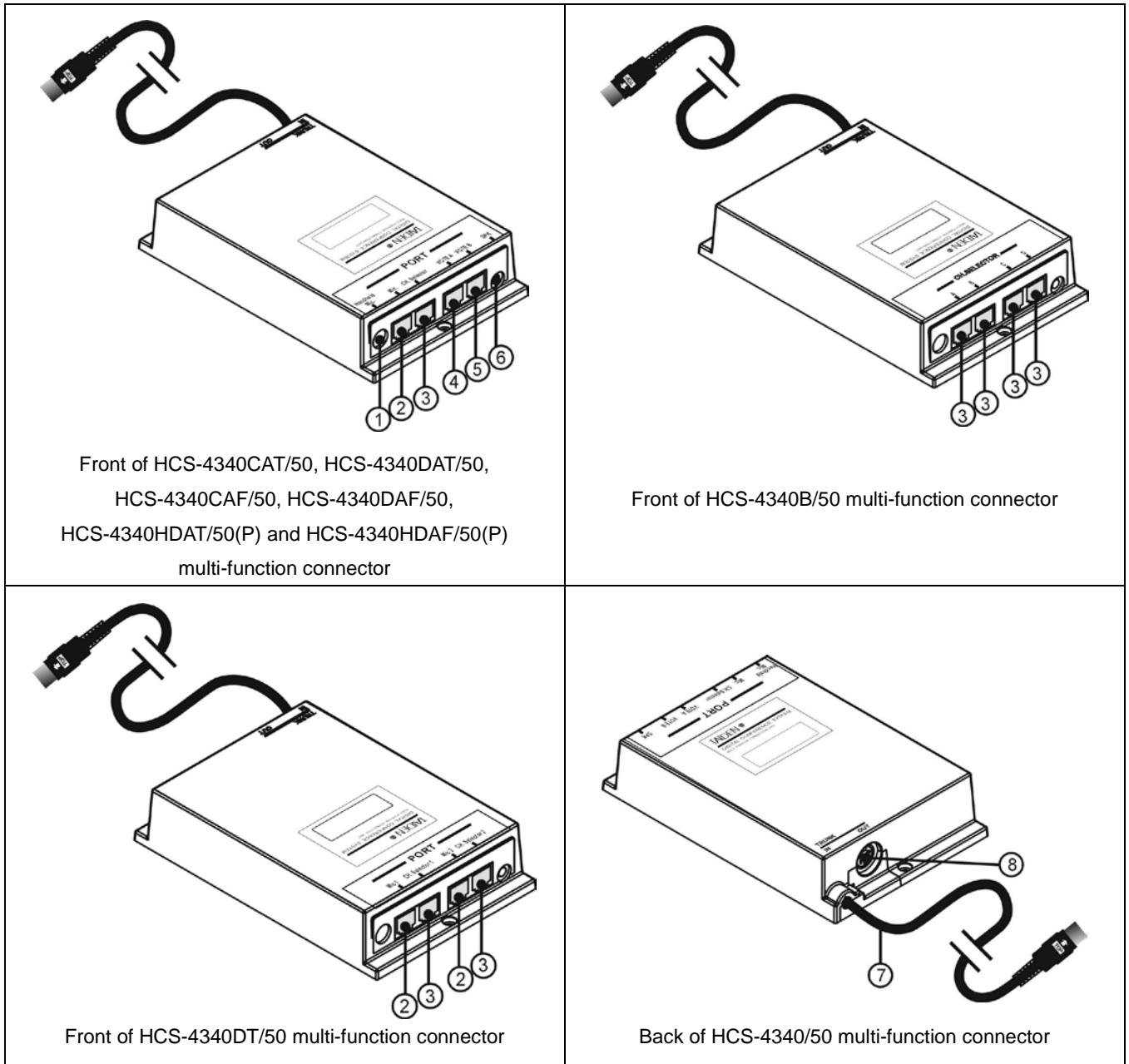
Figure 3.9.2 HCS-4340/50 series multi-function connectors
