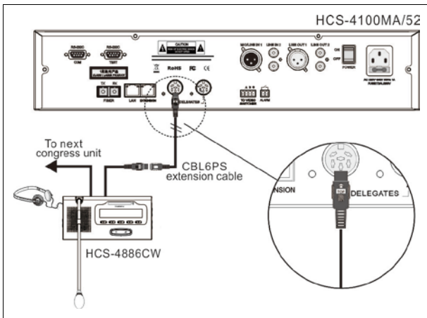
Figure 3.5.2 HCS-4886 series congress unit connected to the CMU/EMU
