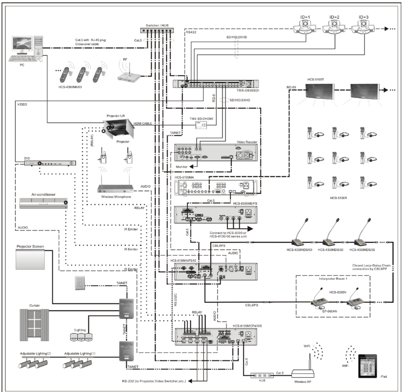
Figure 5.1.5 HCS-4100M/52 congress system main unit connecting to central control system
