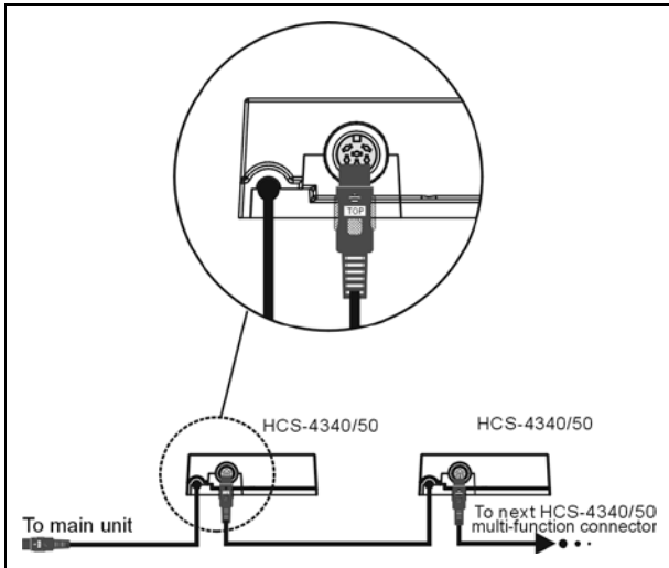
Figure 3.9.4 "Daisy-chain" connection between HCS-4340/50 series multi-function connectors
