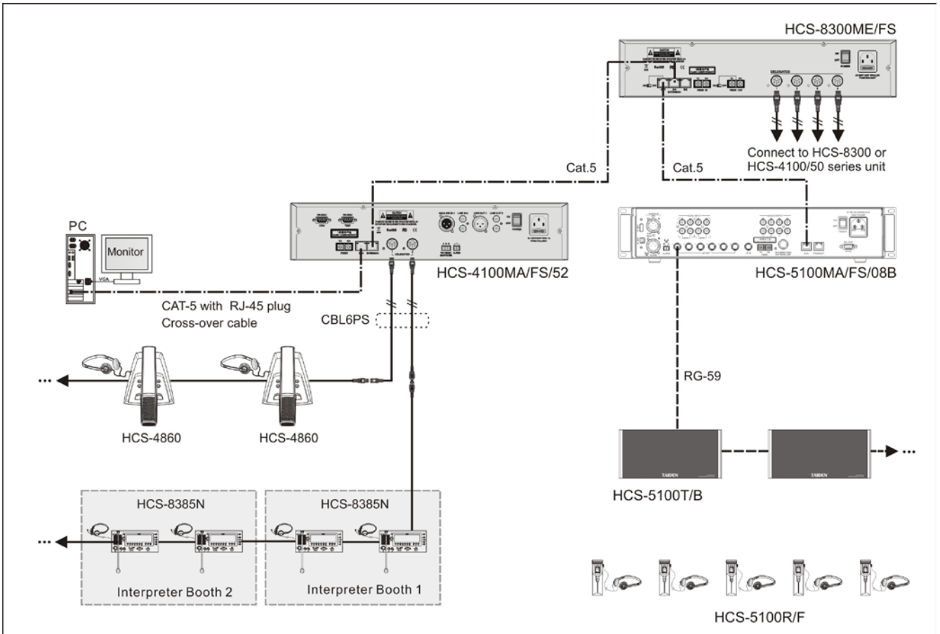
Figure 5.1.3 Congress main unit connecting to digital infrared language distribution system via HCS-5100MA/B
