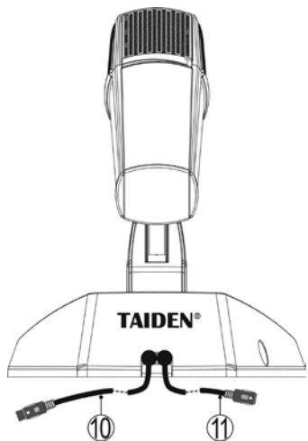
Back of HCS-4860/54
