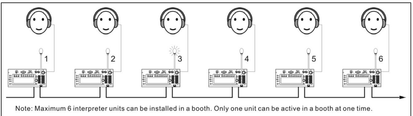
Figure 4.3.3 Schematic diagram of the connection of interpreter units
