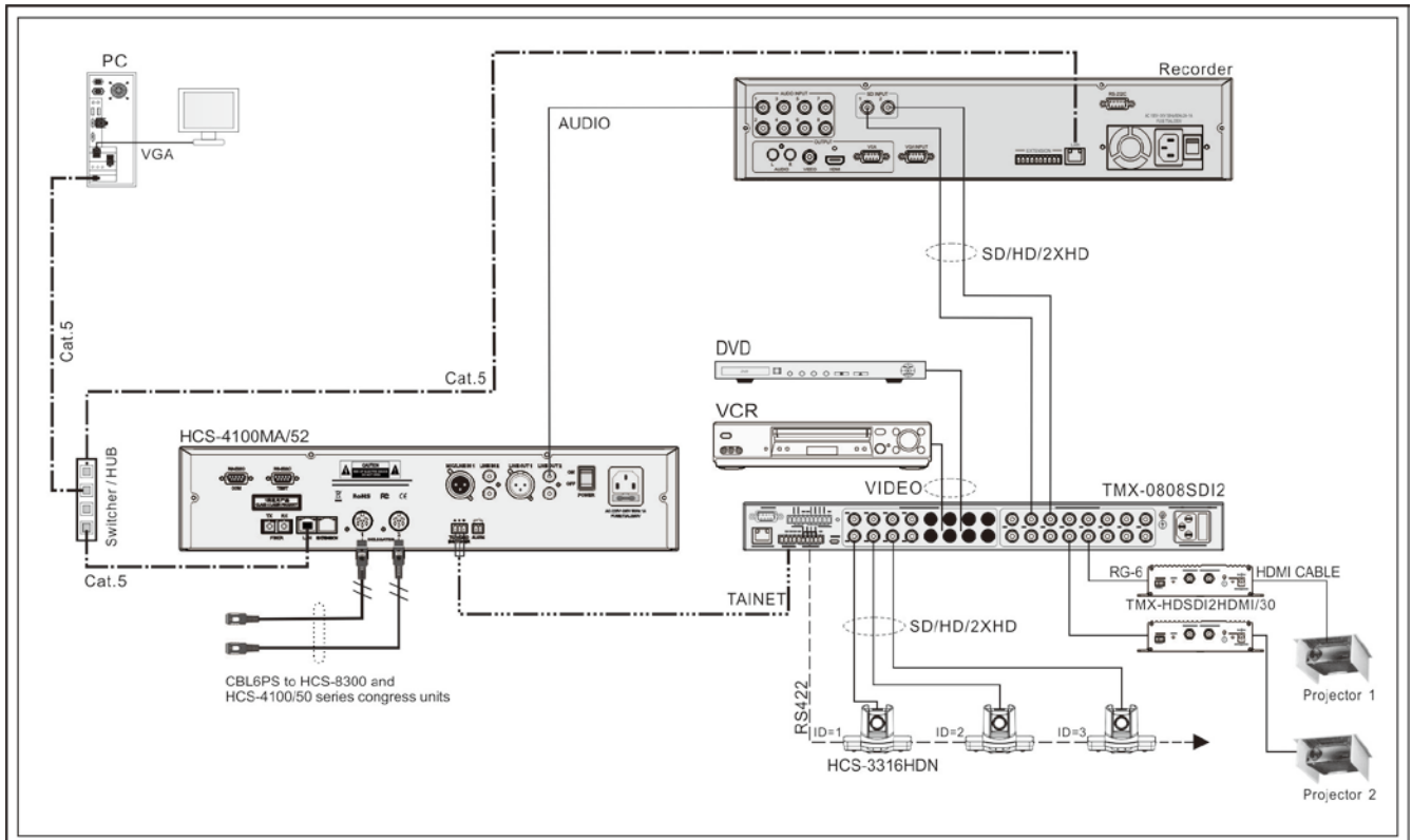
Figure 5.1.2 HCS-4100M/52 congress main unit connecting to the automatic video tracking system
