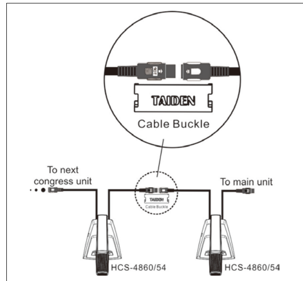
Figure 3.8.3 “Daisy-chain” connection between HCS-4860/54 series congress units
