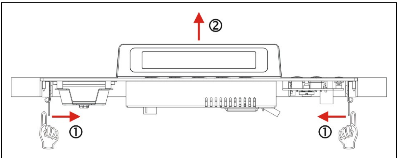
Figure 3.3.8 Disassembly of HCS-48U8 and HCS-48U9 series flush-mounted congress unit (method b)
