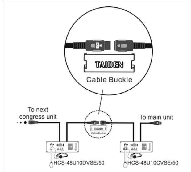
Figure 3.4.5 “Daisy-chain” connection between HCS-48U10/50 series congress units
