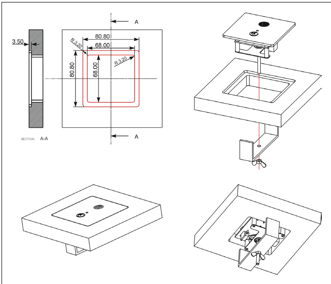
Figure 3.10.5 Installation of the HCS-4841U/50 flush-mounted channel selector
