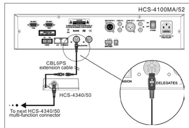
Figure 3.10.7 Multi-function connector connected to the CMU/EMU
