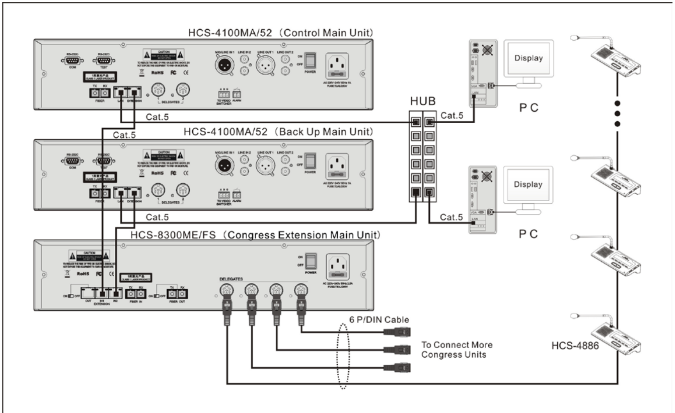
Figure 5.1.8 Dual System Main Unit Hot Spare
