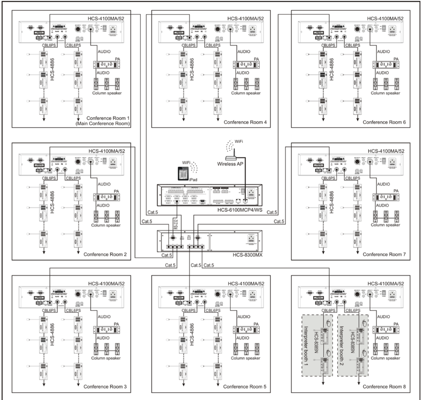
Figure 5.1.7 Combining/splitting meeting rooms with HCS-8300MX Congress Room Combiner and Cat. 5 cables
