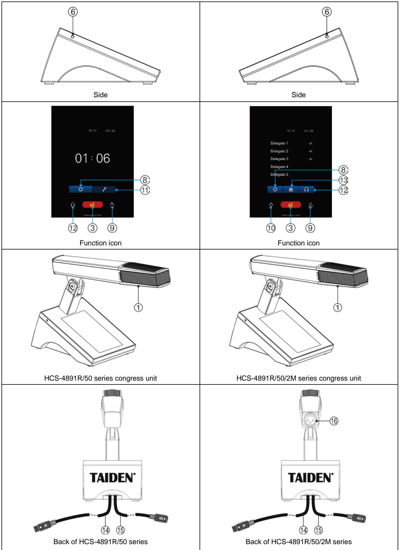
Figure 3.6.1b HCS-4891/50 series congress units
