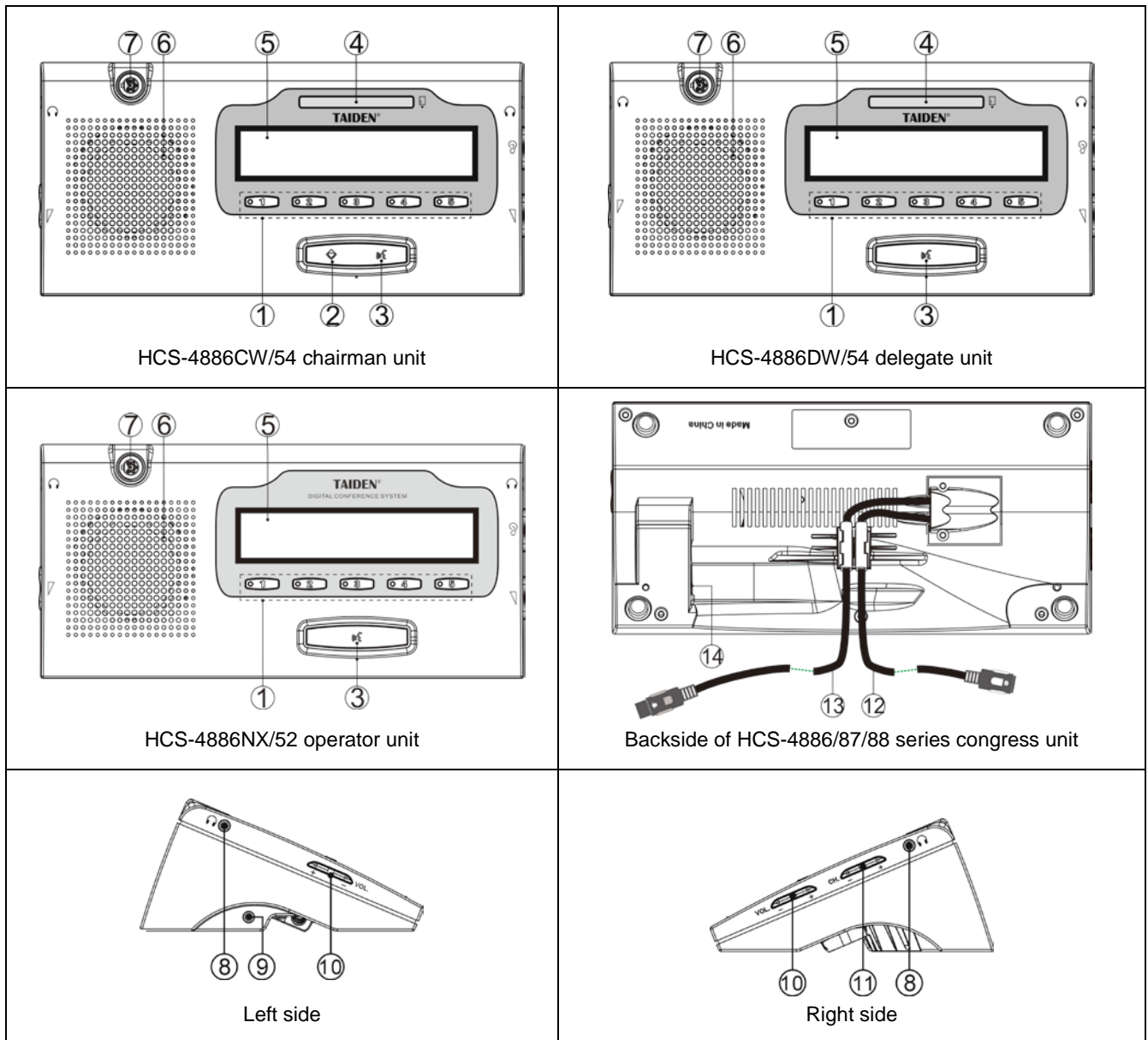
Figure 3.5.1 HCS-4886 series congress units
