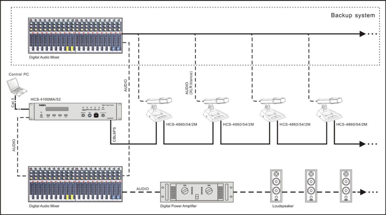
Figure 3.8.4 Dual backup microphone high-end congress system solution
