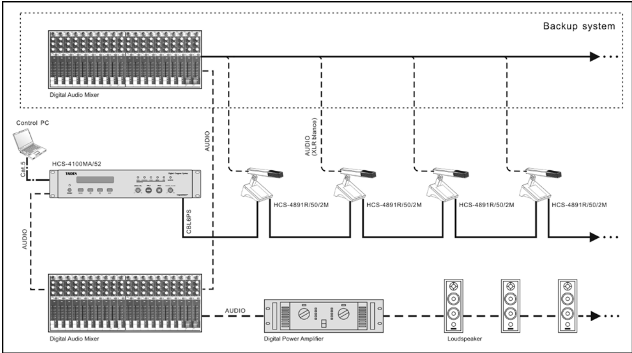
Figure 3.6.4 Dual backup microphone high-end congress system solution
