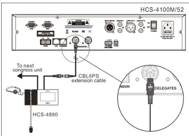
Figure 3.6.2 HCS-4890/52 series congress unit connected to the CMU/EMU
